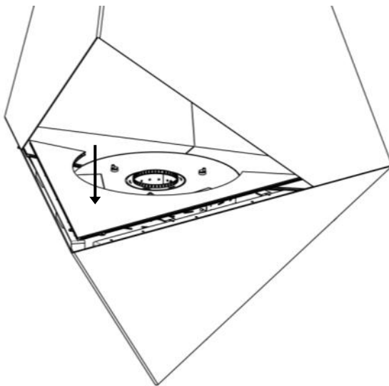
Figure 10 - Placement of decorative plate
