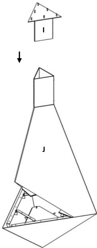
Figure 2— Fixing tube assembly
