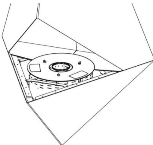
Figure 9 - Burner placed in the fireplace
