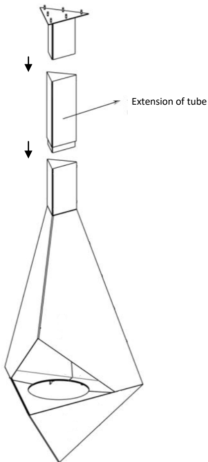
Figure 13— Placing the extension of tube
