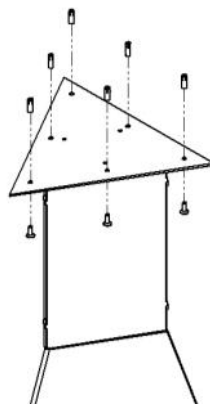
Figure 5 - Top part to screw to the ceiling
