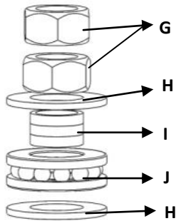
Figura 3— Assembly order
