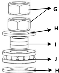
Figura 3— Assembly order
