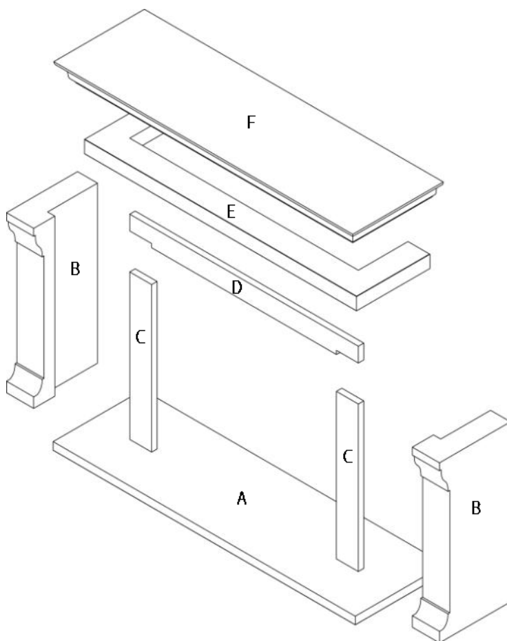
Figure 8 - Stone fireplace components
