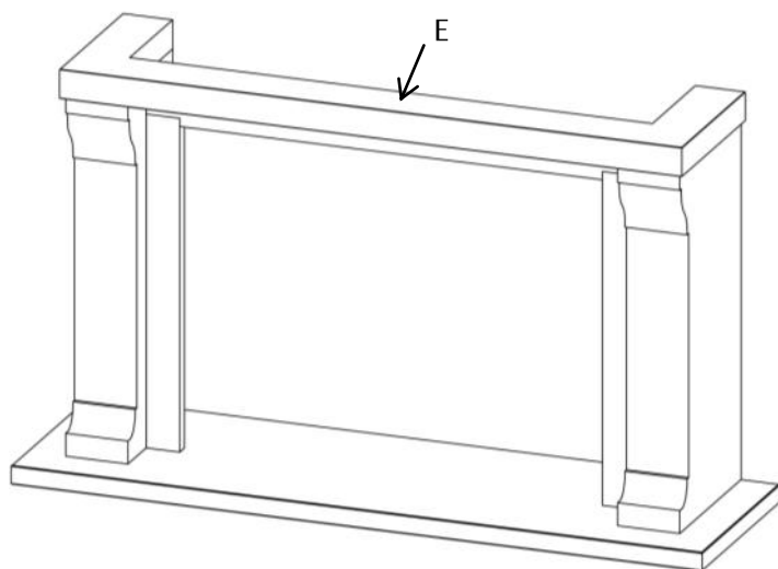
Figure 12 – Placing the stone E .
