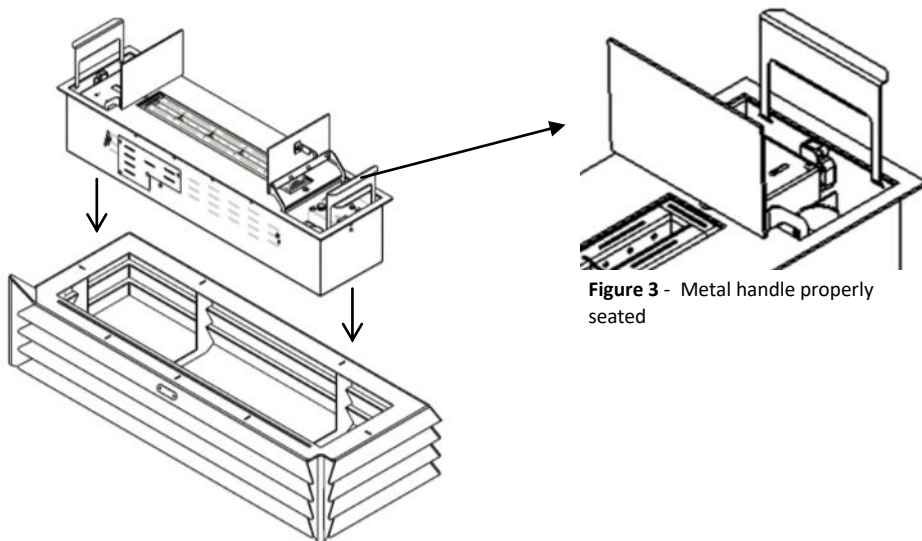
Figure 2 - Placing the burner
