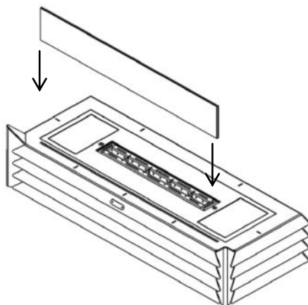
Figure 4 - Placing the glass
